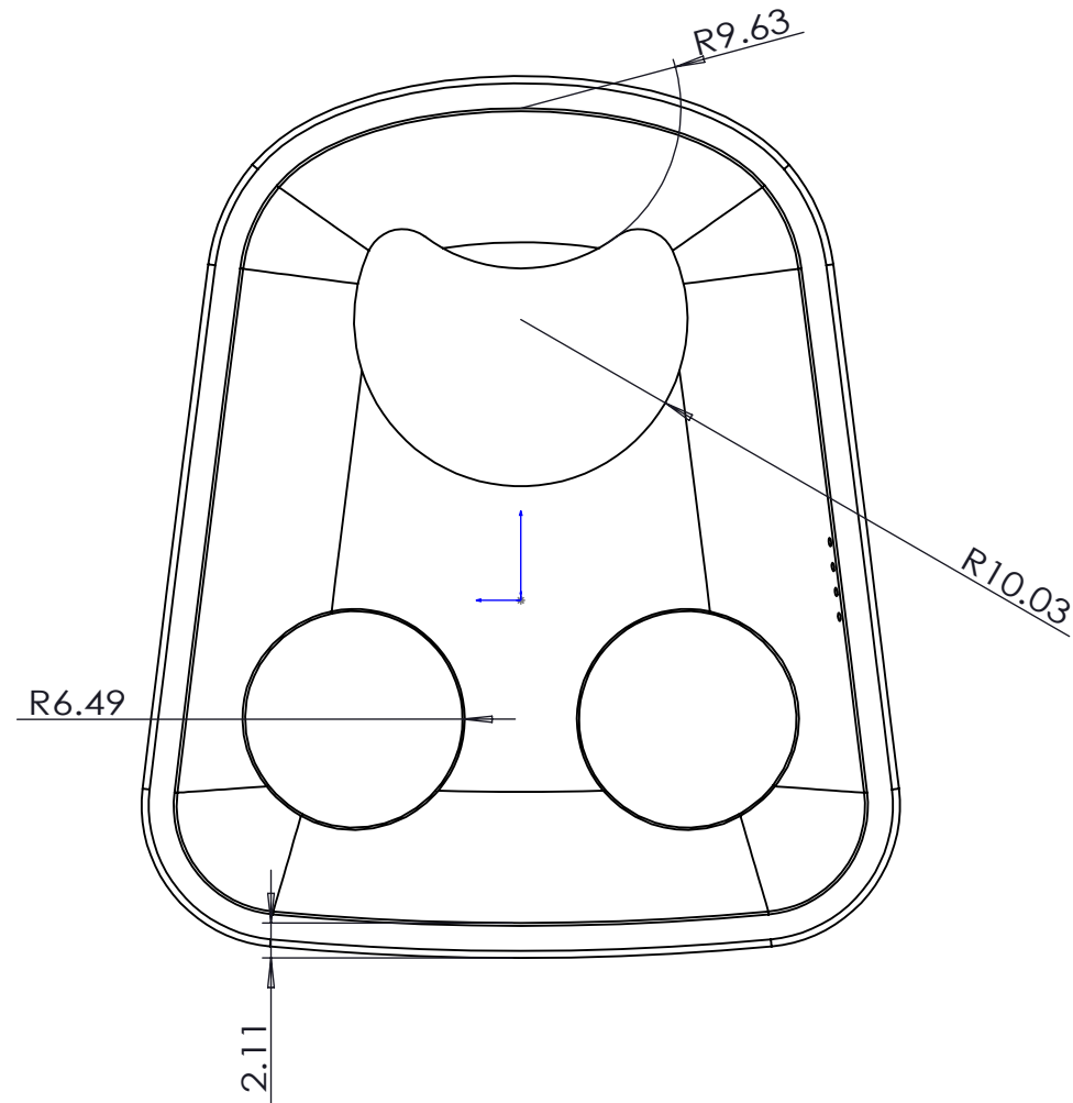
BACK VIEW
