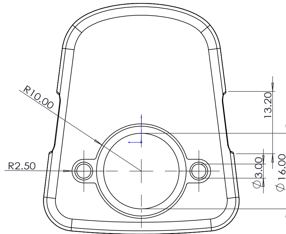
BACK VIEW
