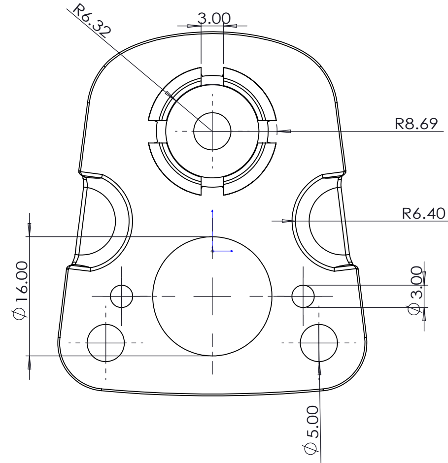
FRONT VIEW
