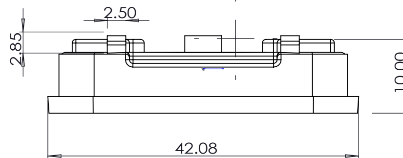
BOTTOM VIEW
